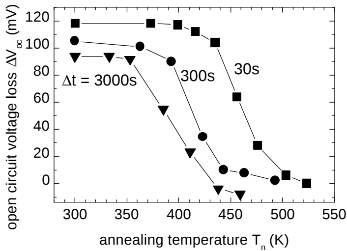
Figure 1 : The decrease of the open circuit voltage loss \Delta V_{OC} towards zero with stepwise increased annealing temperature T_n shows that, after sufficient annealing, the devices completely recover from the radiation damage. The time steps \Delta t for the isochronal annealing experiments in air are \Delta t = 3000 s (triangles), 300 s (circles), and 30 s (squares).
