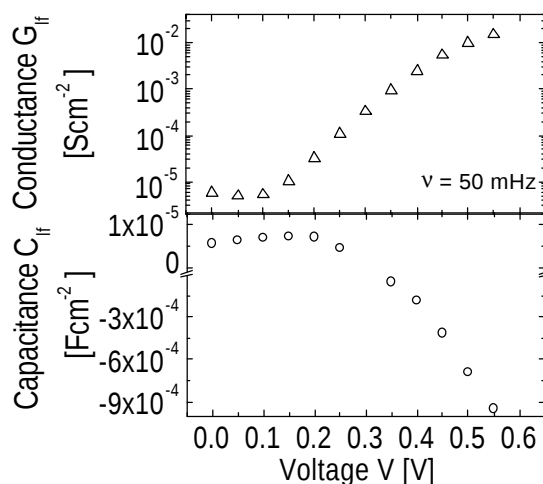
Figure 2: The low-frequency conductance G_{If} of the solid-state DSSC increases exponentially under forward bias V whereas C_{If} becomes negative for voltages V > 0.3 \text{ V} .
