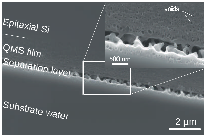
Figure 1: Cross section scanning electron microscopy picture of the double-layer porous structure after restructurization. The small picture shows a detail of the separation layer and the QMS film.
