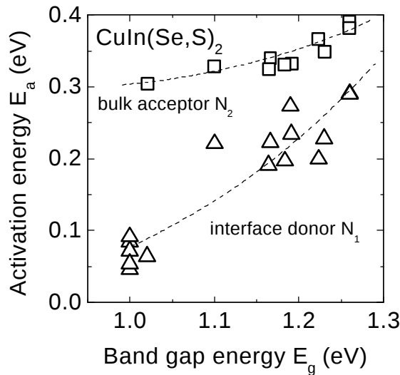
Figure 1: The activation energies of the interface donor N_1 and the bulk acceptor N_2 increase with increasing band gap energy, if \text{CuInSe}_2 is alloyed with S. Dashed lines are guides to the eyes.
