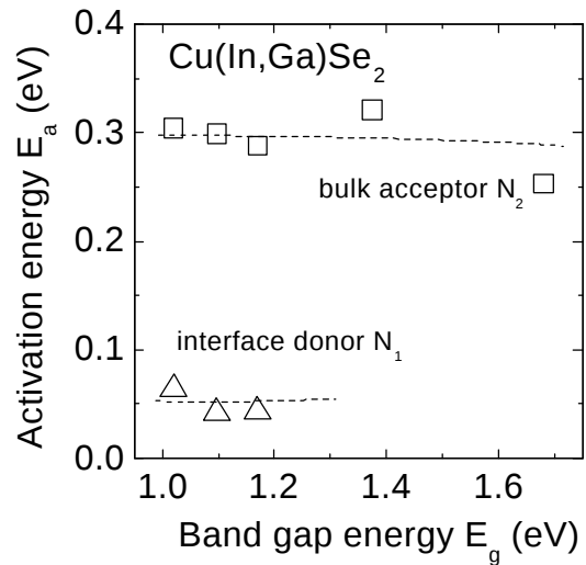
Figure 2: The activation energies of N_1 and N_2 remain constant, if the band gap of \text{CuInSe}_2 is increased by alloying with Ga.
