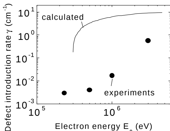
Figure 1: Defect introduction rate for electron irradiation: Theoretical values (solid line) calculated from the displacement cross section and experimental results (solid symbols).
