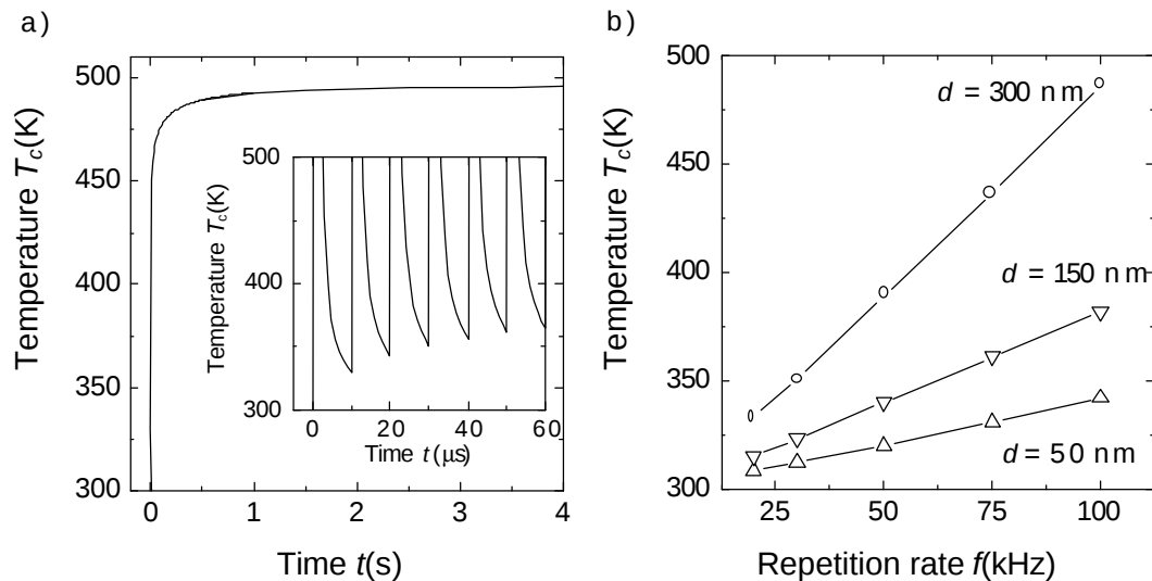
Figure 1: a) Surface temperature T_c of a 300 nm thick silicon film versus time. During the first laser pulses T_c increases very rapidly and begins to saturate after approx. 0.5 s. Inset graph displays the temperature evolution during the first six laser pulses. b) Saturated surface temperature of silicon films with different thicknesses in dependence of the repetition rate of the laser.
