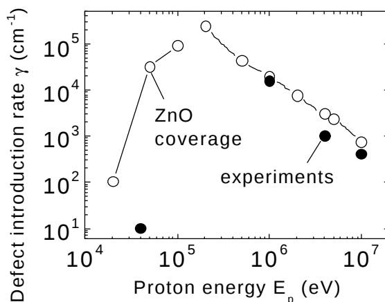
Figure 2: Defect introduction rate of protons in CIGS obtained by TRIM simulations (open symbols) and determined by irradiation experiments (solid symbols).
