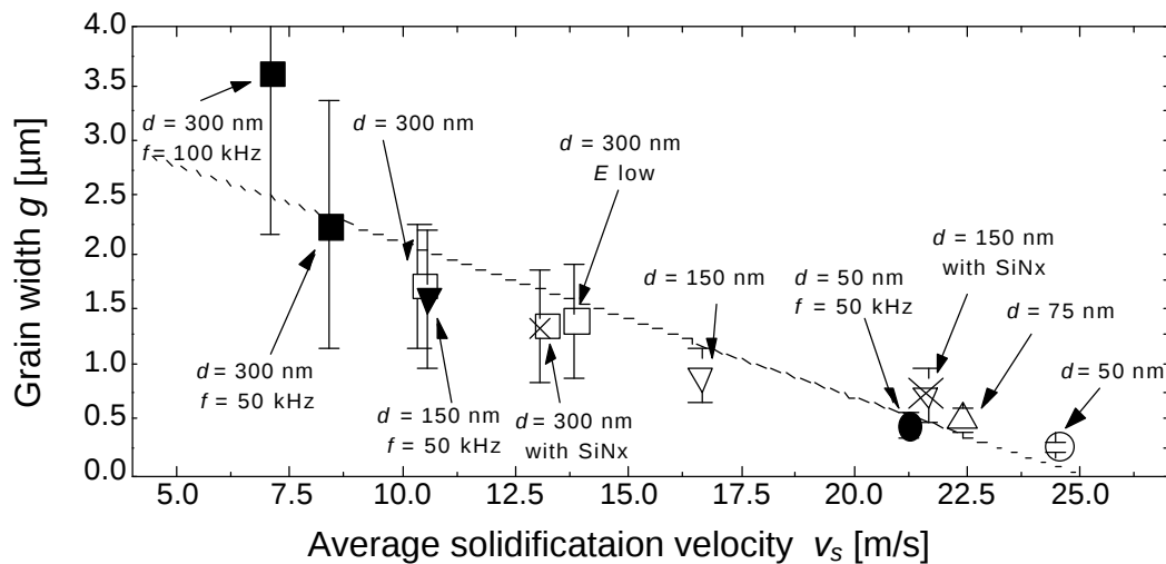
Figure 2: Solidification velocity v_s is extracted from numerical simulations. Data points without a stated f -value hold for f = 20 kHz. Error bars indicate the standard deviation of the grain width distribution. The dotted line is a linear fit to the data points.
