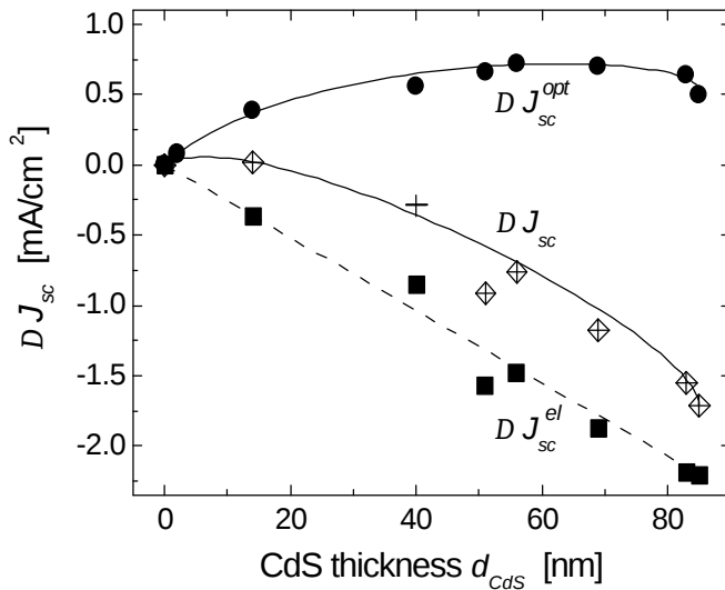
Figure1: Optical gain \Delta J_{sc}^{opt} (circles), electronic loss DJ_{sc}^{el} (squares), and the total current density change DJ_{sc} (crossed diamonds). The upper two datasets are connected with spline curves as guides to the eye, the electronic loss follows a linear fit. Optical gain and electronic loss almost compensate each other for CdS thicknesses between d_{CdS} \gg 0 and 40 nm.
