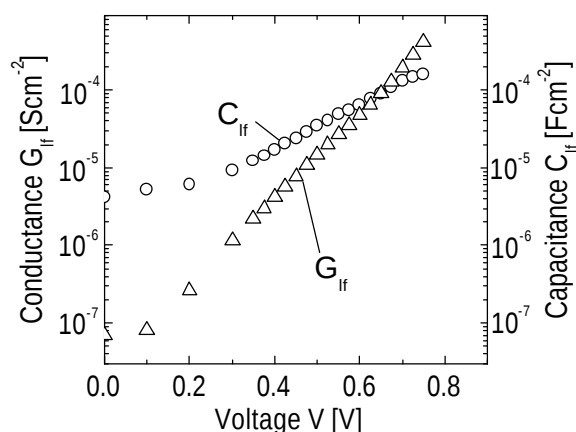
Figure 1: The exponential increase of the low-frequency capacitance C_{If} and of the conductance G_{If} is explained by the injection and diffusion of electrons in the \text{TiO}_2 .
