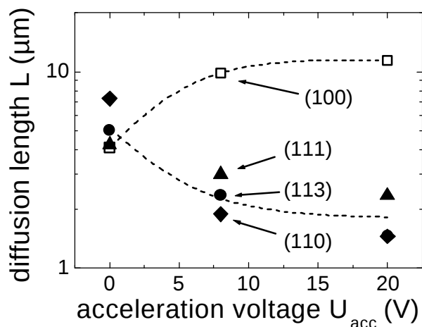
Figure 1: Influence of ion energy on the minority carrier diffusion length L of films deposited at T_{dep} = 650^{\circ}C . In the case of (100)-oriented films an increase of the acceleration voltage from 0 V to 8 V results in an increase of L by more than a factor of two. However, for non-(100)-oriented films the minority carrier diffusion length decreases with rising ion energy.
